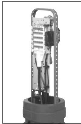
MAH77 Shown With 25-Pair Mini-Rocker Terminal Block
