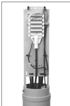
CFP800 Shown With 25-Pair Mini-Rocker Terminal Block
